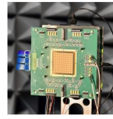
Anokiwave 256 elements
